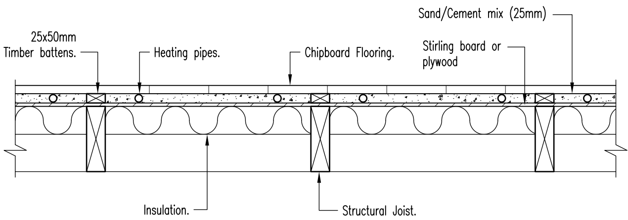
Underfloor Heating On A Suspended Timber Floor
